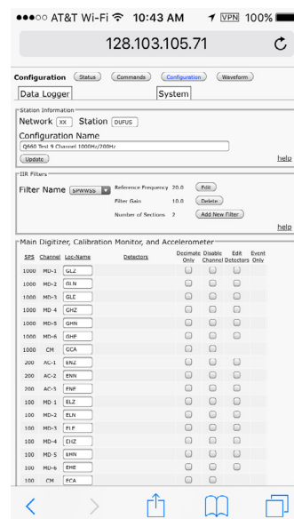
iPhone™ Screenshot showing one of the MSED channel-configuration pages, connected via WiFi
